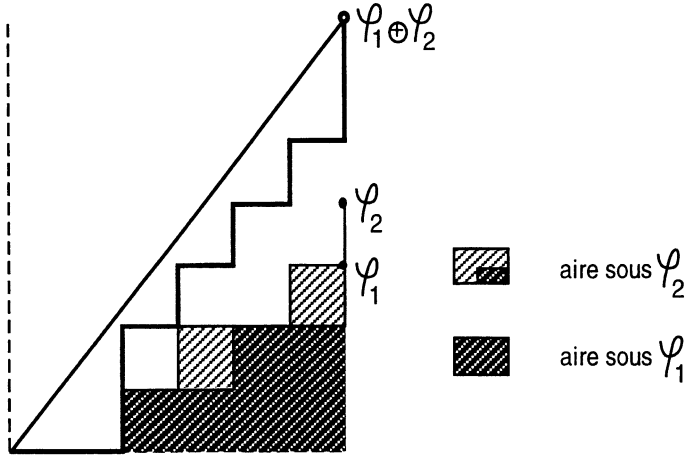
Figure 4 : addition. 001001001 \oplus 0010100101 = 0011010101011 .
